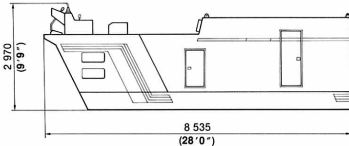
Engine unit (left); 15 700 kg (34 600 lb)
