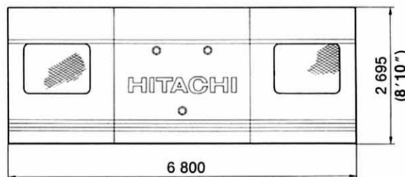
Counterweight; 40 500 kg (89 300 lb)
