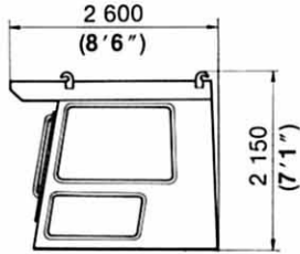
Cab; 880 kg (1 940 lb)
