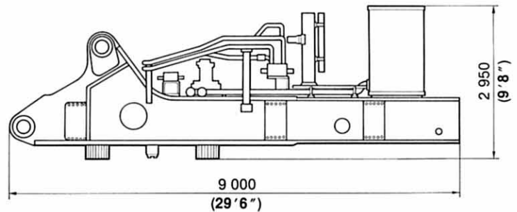
Main frame assembly; 45 440 kg (100 200 lb)
