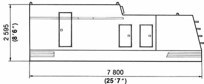
Engine unit (right); 17 300 kg (38 100 lb)
